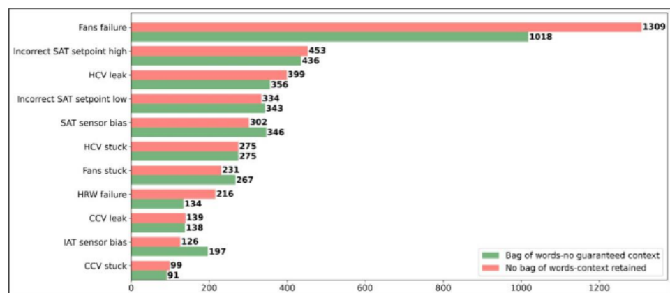
Figure 4: Results for fault frequency occurrence obtained through network clustering for both cases (with and without applying the bag of words feature).
